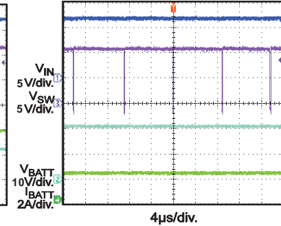
Power Off V_{BATT} = 10.8V
