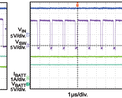
Power On V_{BATT} = 10.8V
