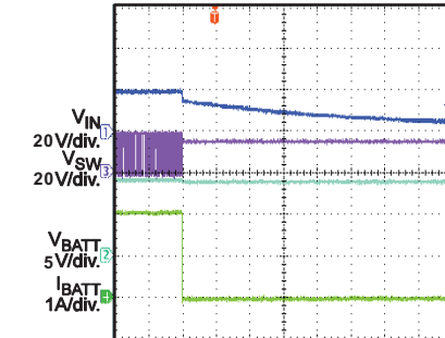
Power Off V_{BATT} = 10.8V
