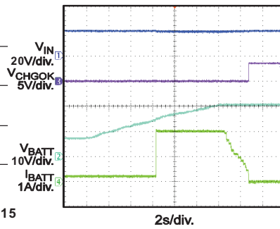
CC Steady State V_{BATT} = 10.8V
