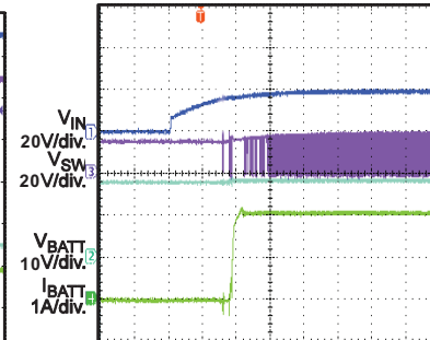
Power On V_{BATT} = 10.8V
